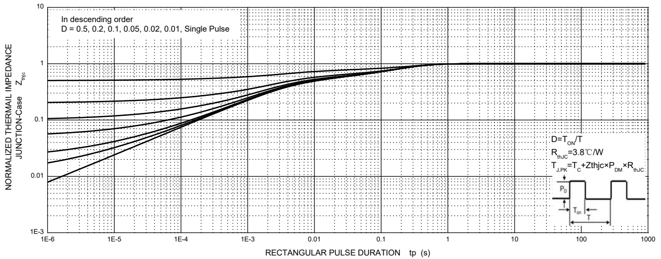
MURF1060CT Transient Thermal Impedance, Junction-Case
