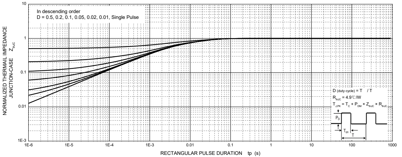
MURF10H20CT Transient Thermal Impedance, Junction-Case
