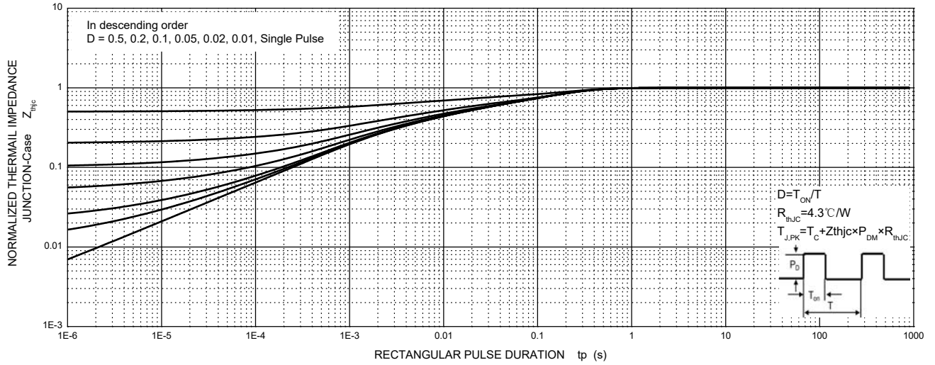
MURF10H60 Transient Thermal Impedance, Junction-Case
