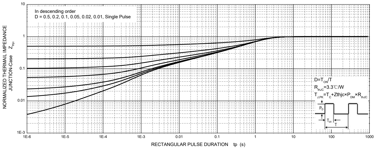
MURF15H60 Transient Thermal Impedance, Junction-Case
