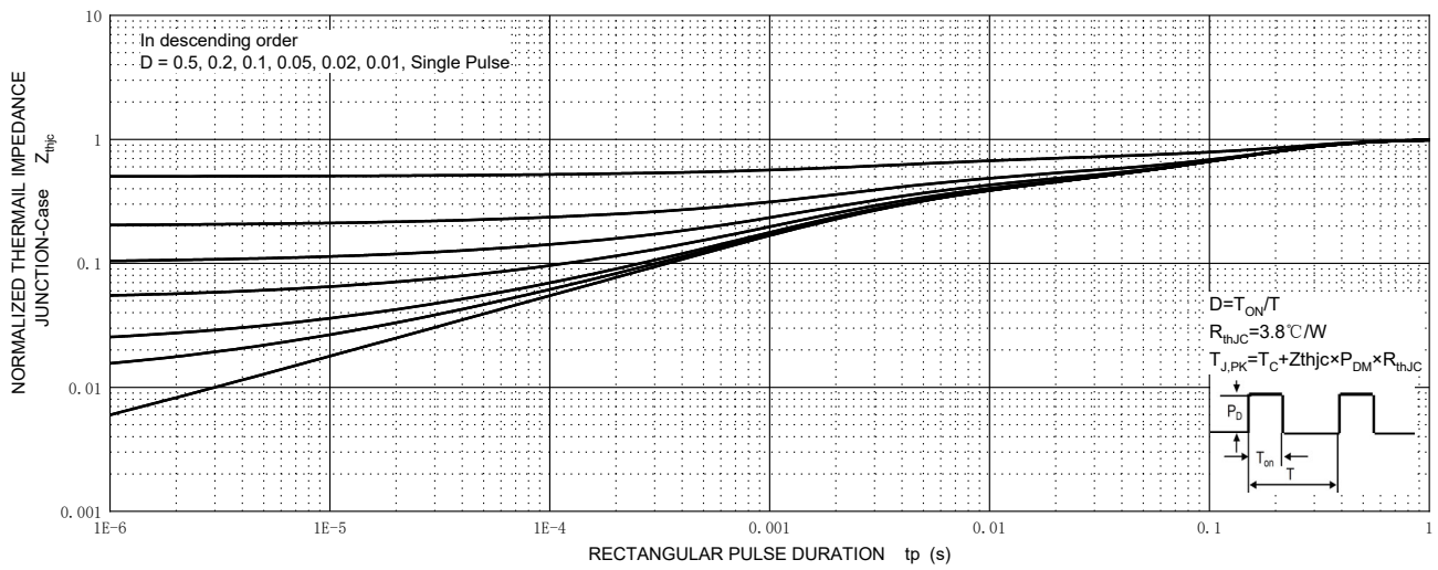
MURF1660CT Transient Thermal Impedance, Junction-Case
