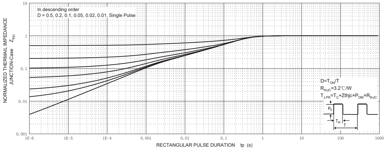
MURF20H65L Transient Thermal Impedance, Junction-Case
