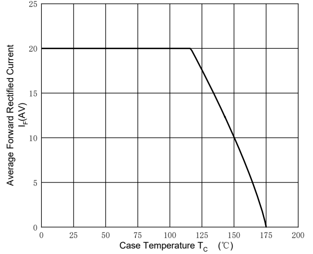
Current Derating
