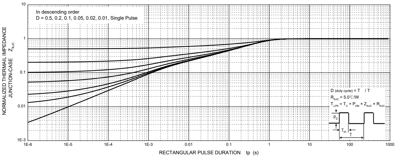
MURF30H60CTB Transient Thermal Impedance, Junction-Case
