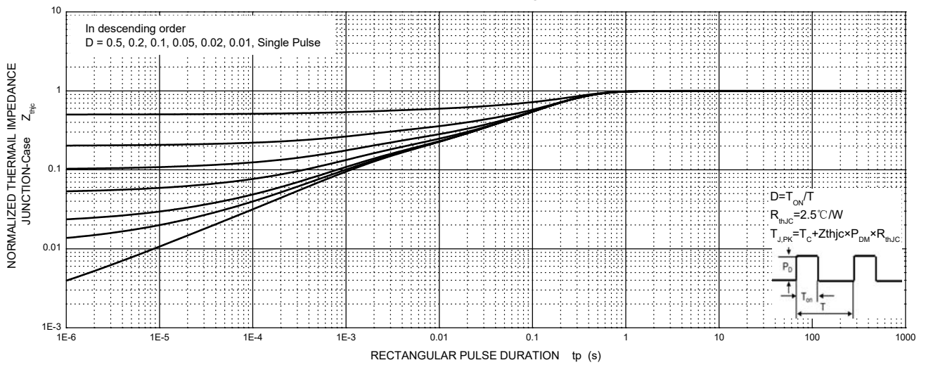
MURF30H60L Transient Thermal Impedance, Junction-Case
