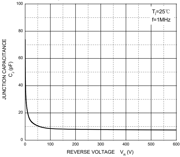
Capacitance Characteristics
