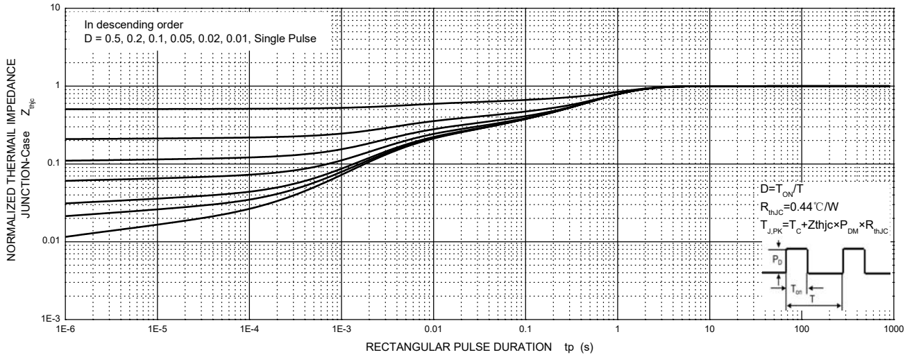
MURW60H120 Transient Thermal Impedance, Junction-Case
