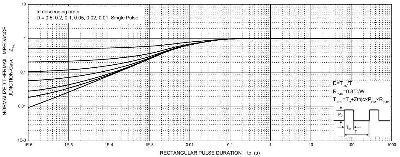
MURW60H20LCTB Transient Thermal Impedance, Junction-Case
