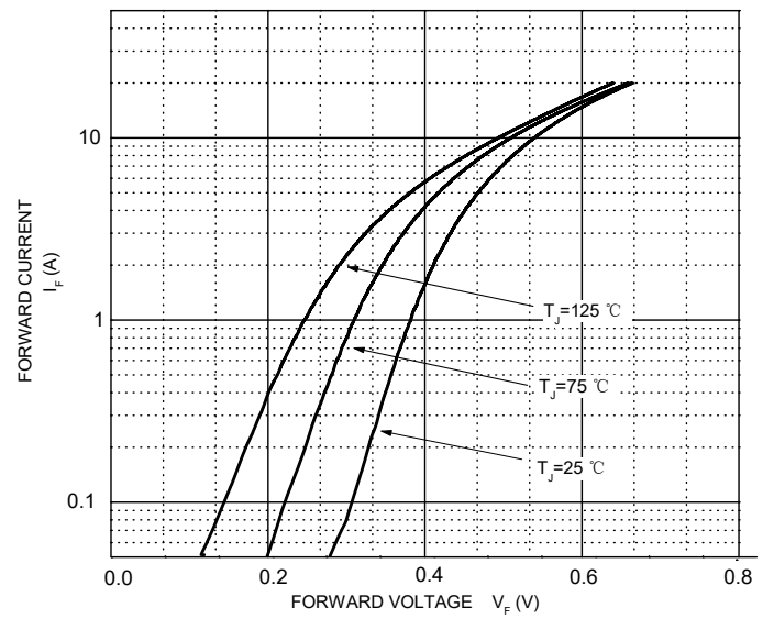
Forward Characteristics
