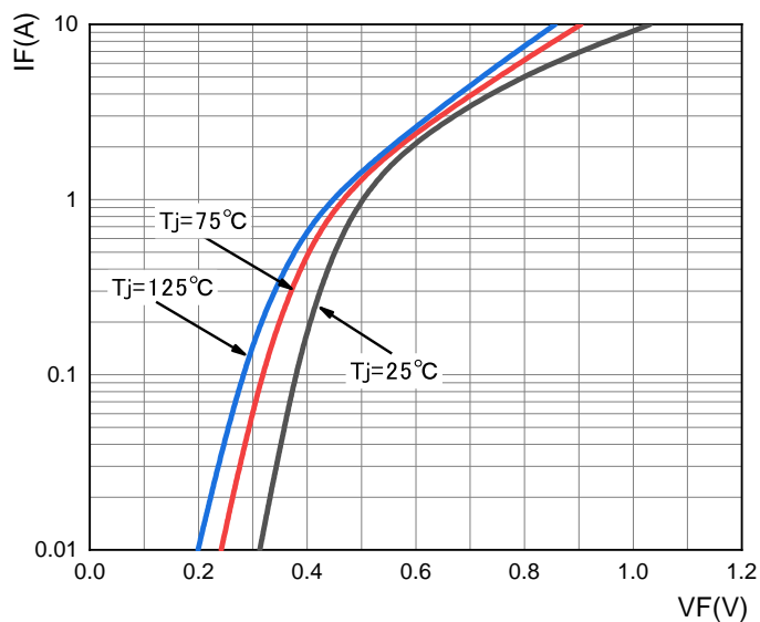
SS12-SS14 FIG.3: TYPICAL FORWARD CHARACTERISTICS
