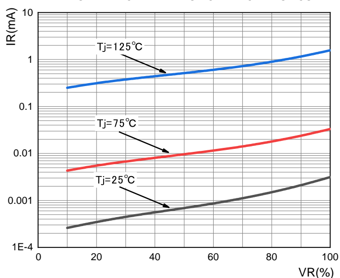
SS12-SS14 FIG.4: TYPICAL REVERSE CHARACTERISTICS
